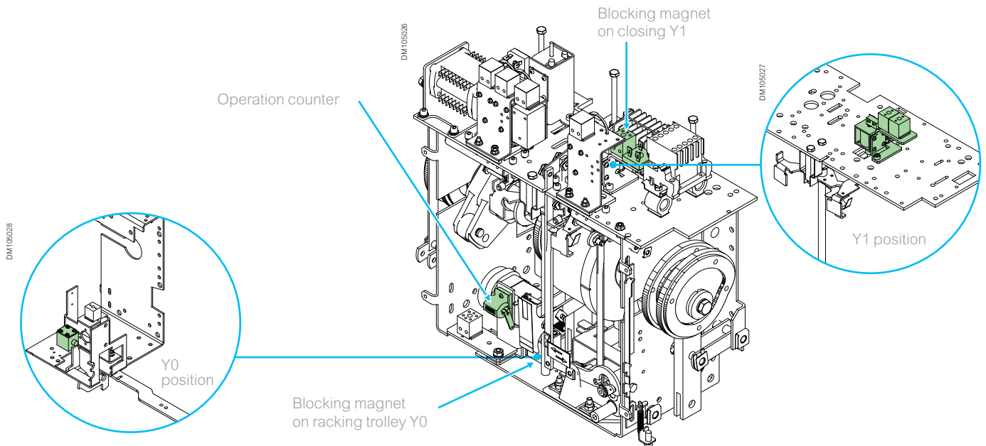
Operation counter
