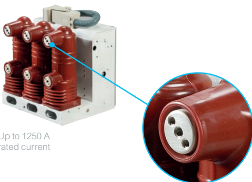
Fixed type
