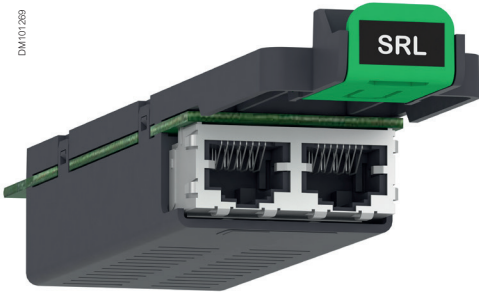
RS485 serial line module
