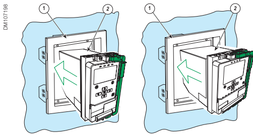
Assemble the flush mounting accessory (1) and the case (2)
